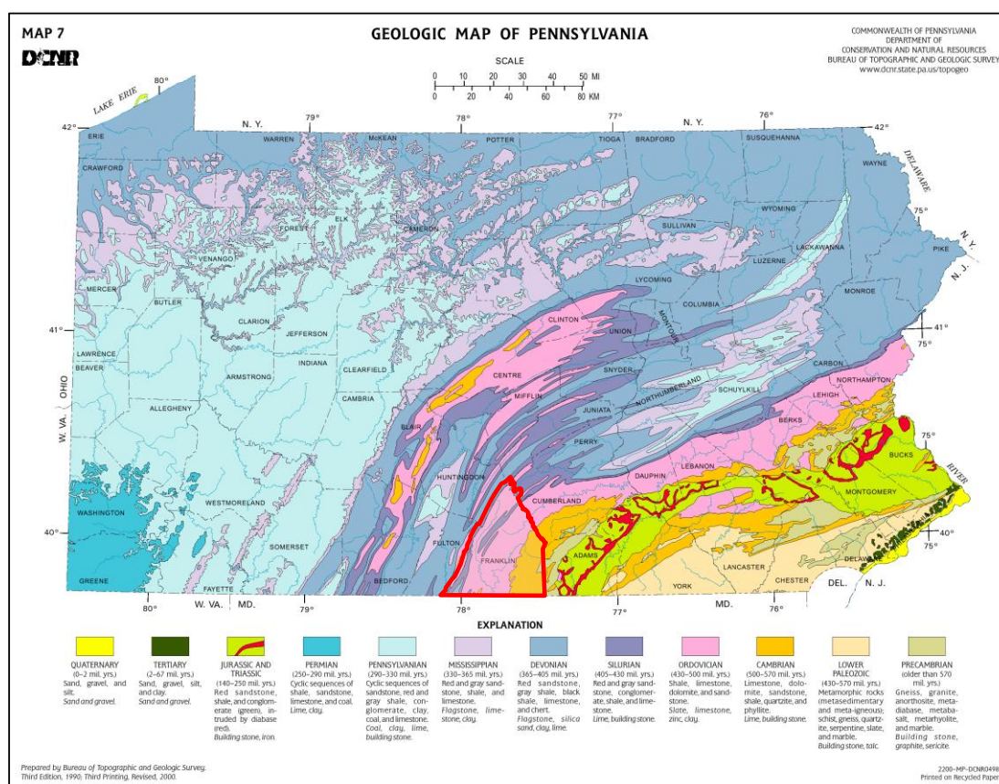
Figure 3.1.20.2.1: Geologic Map of Pennsylvania (2000) 142
