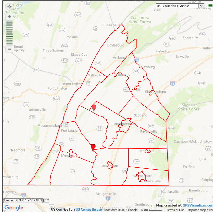
Figure 3.1.20.3.2: Location of Caves in Franklin County (2017) 144
