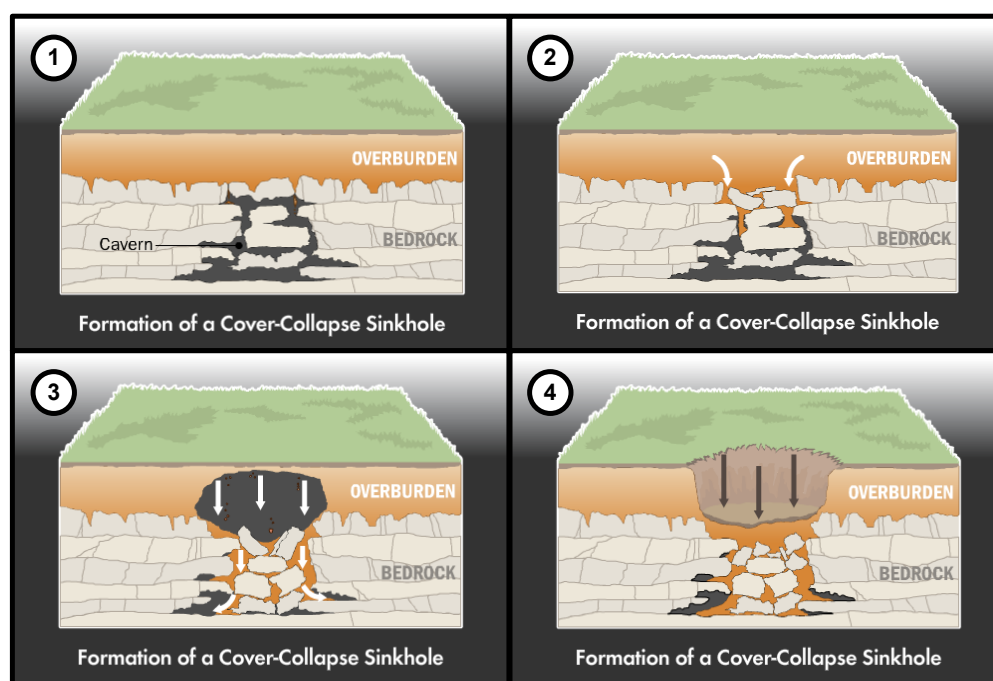
Figure 3.1.20.1: Formation of a Collapse Sinkhole 139
