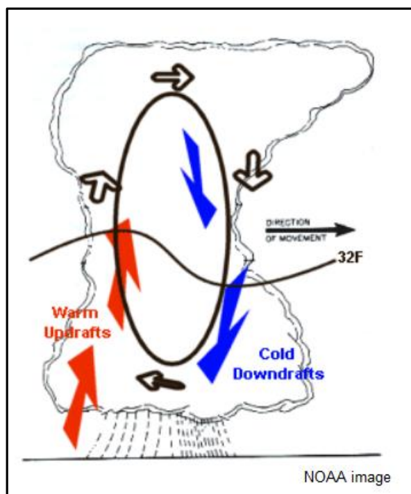
Figure 3.1.10.1: Hail Formation
