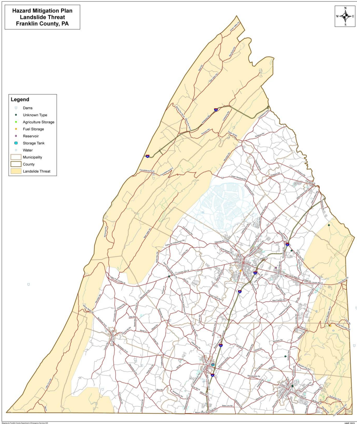
Figure 3.1.13.2: Areas of Landslide Susceptibility of Franklin County (Mar 2023)
