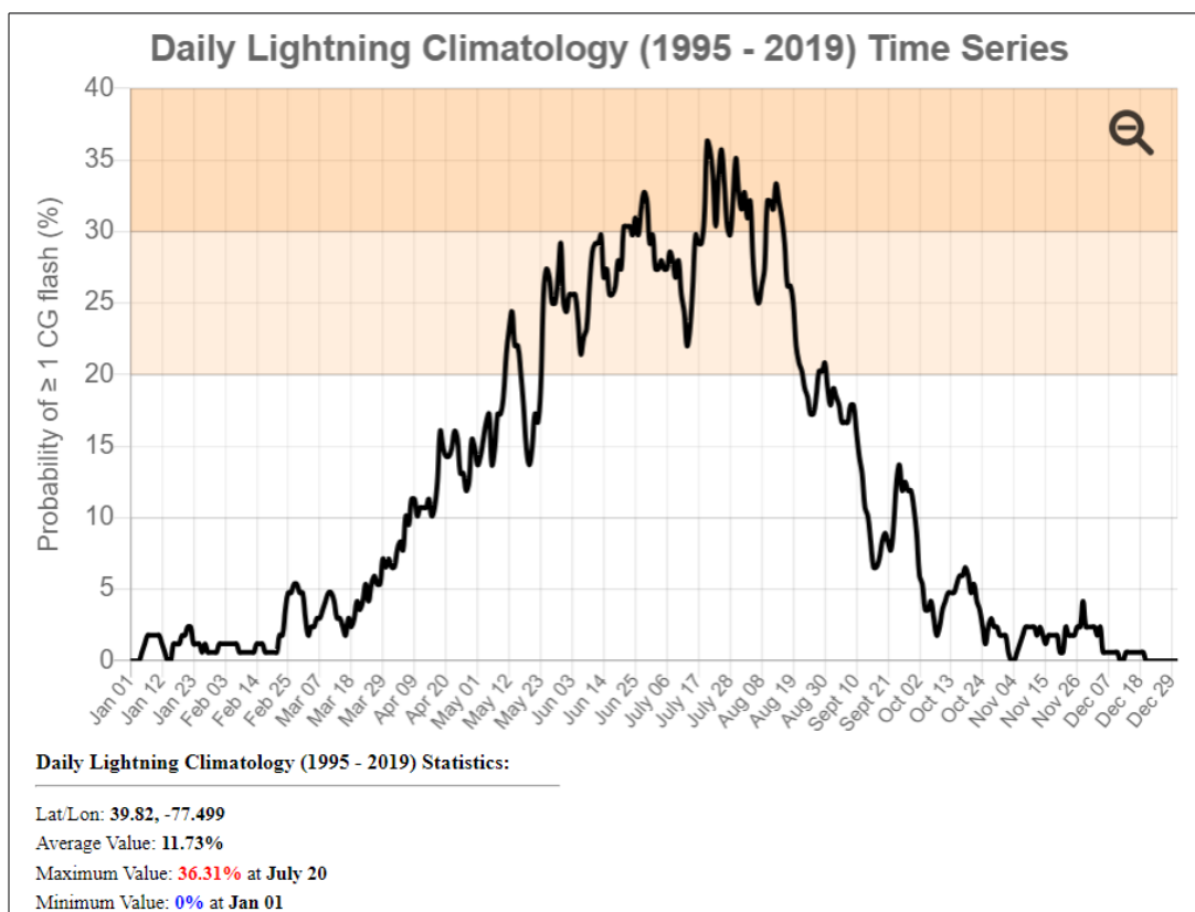
Figure 3.1.14.3.2: NOAA Annual Probability of Cloud to Ground Lightning Flashes
