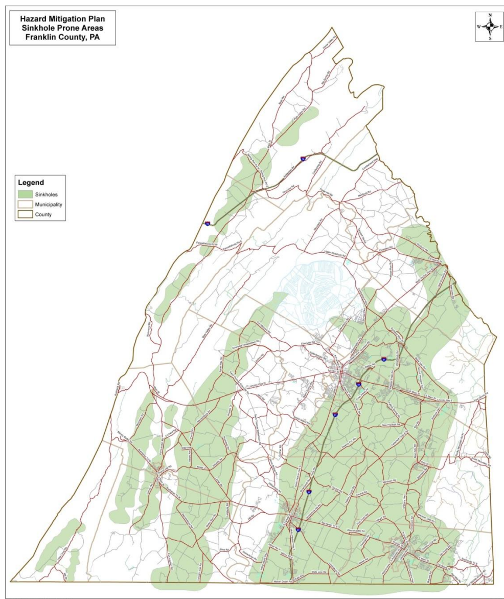
Figure 3.1.20.4.1: Areas of Susceptibility to Sinkholes in Franklin County (Mar 2023)
