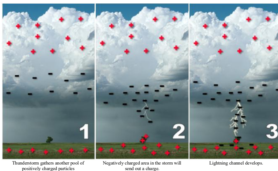
Figure 3.1.14.1: Formation of Lightning 99
