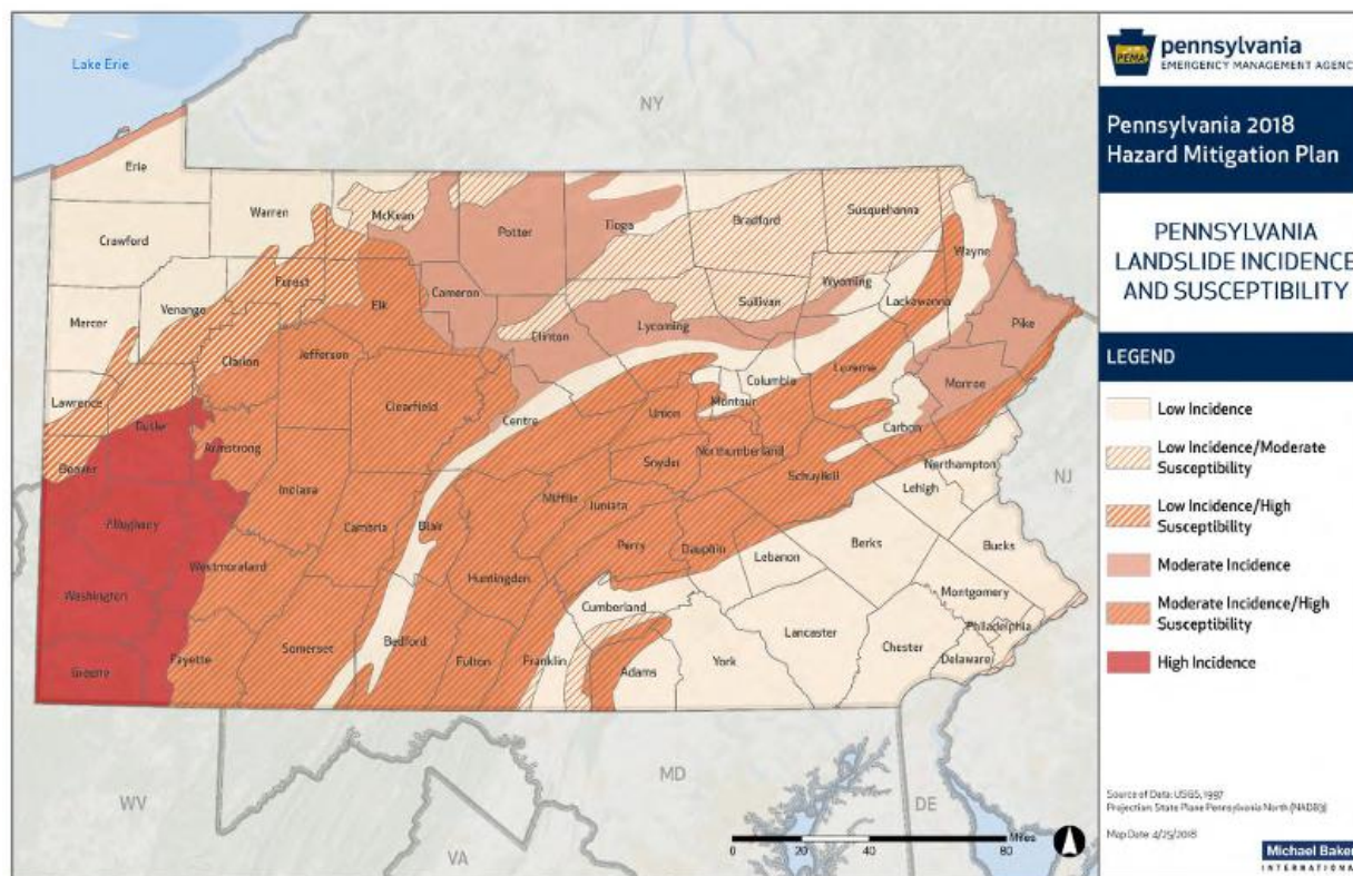
Figure 3.1.13.1: Landslide Susceptibility in Pennsylvania 96
